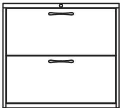
Lateral File - 2 High W 30 D 18 H 27 Available as 3, 4 or 5 high. 30", 36" and 42" W available.
